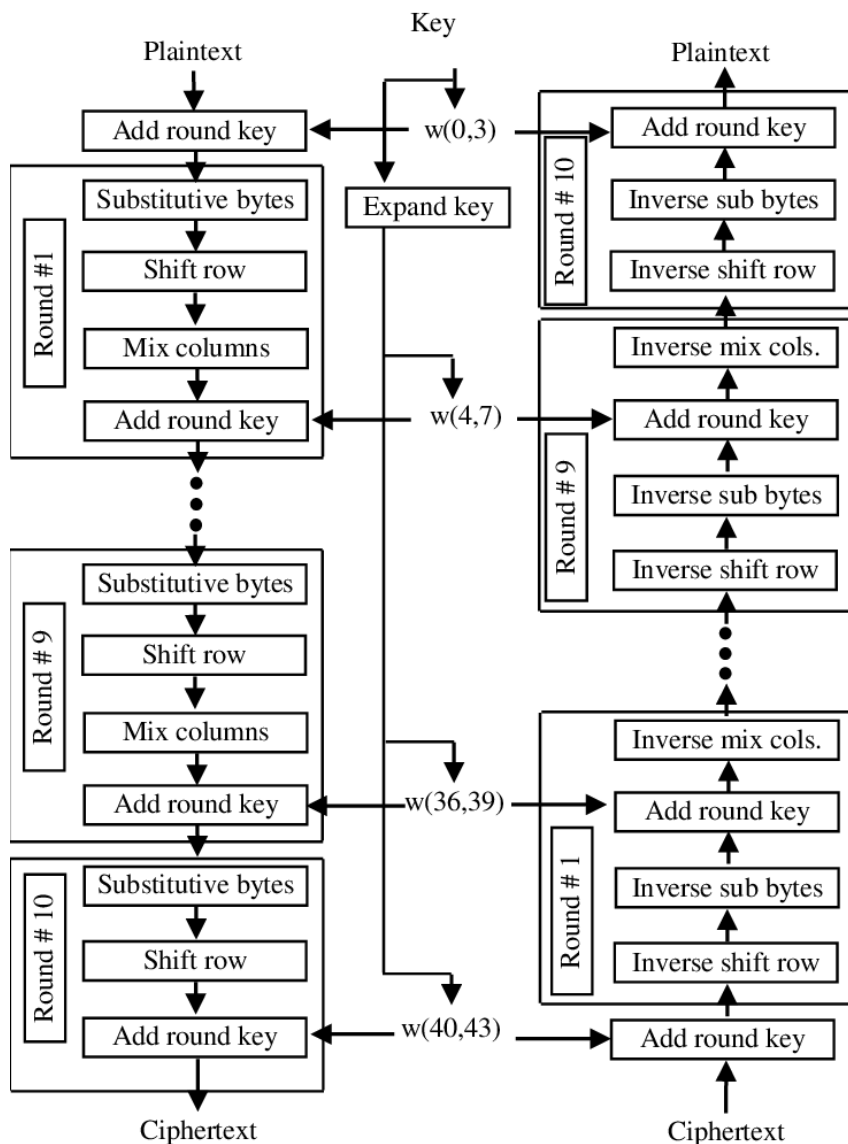
Figure 1: Overview of the AES algorithm.
